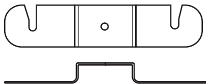
Connecting plate
